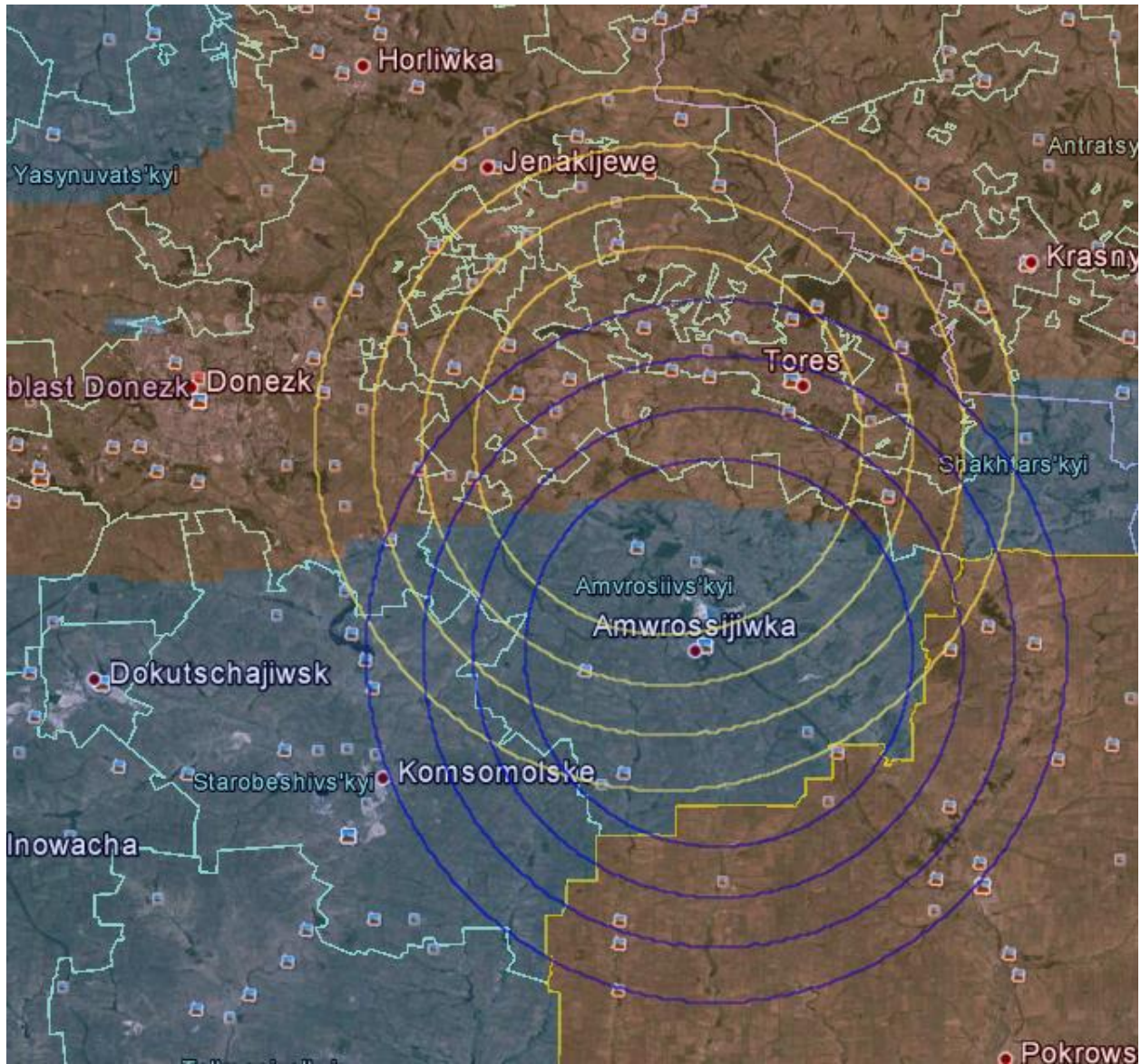
Figure 19: Engagement zone of a Buk M1; Circles are at approximately 20, 25, 30, and 35 kilometers from the Buk M1 position; Yellow: Center of Almaz-Antey launch site; Blue: Amvrosiivka field camp; Situation map from Kot Ivanov's blog from 15 to 18 July 2014 was used for an estimation of the area under control; Blue area: Ukrainian control; Red area: Russian control; The western and northern areas are only a rough approximation
