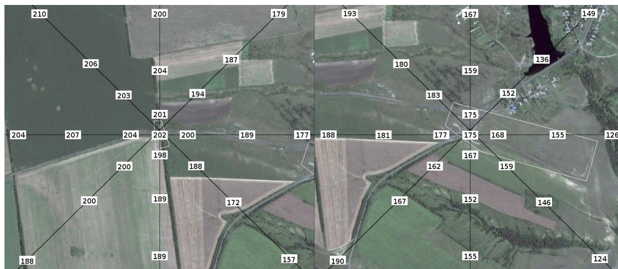
Figure 12: Southern fortifications near Velyka Shyshivka and elevation of selected places around the positions: Left: west fortification; Right: middle (and right) fortification
