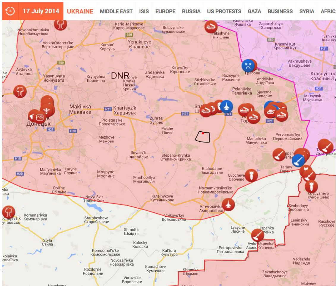
Figure 6: LiveUAmaph situation map, 17 July 2014; Area outlined in black: Almaz-Antey launch site; Red square: Russian MoD site; Source: http://liveuamap.com/
